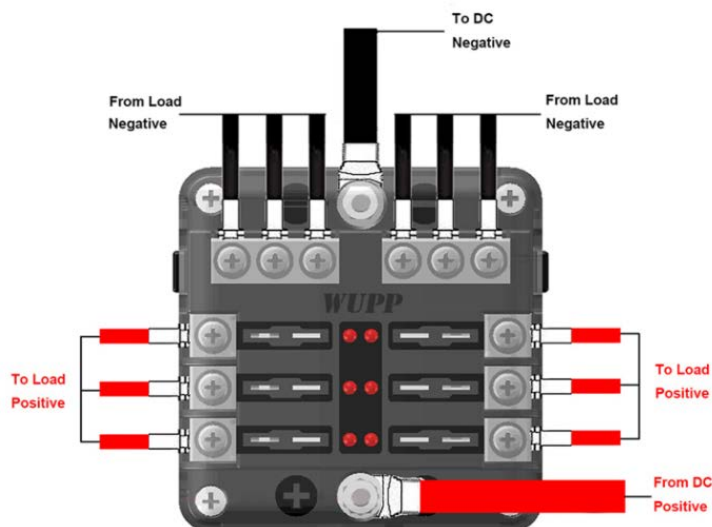
Figure 1. Fuse Holder – Reference only
